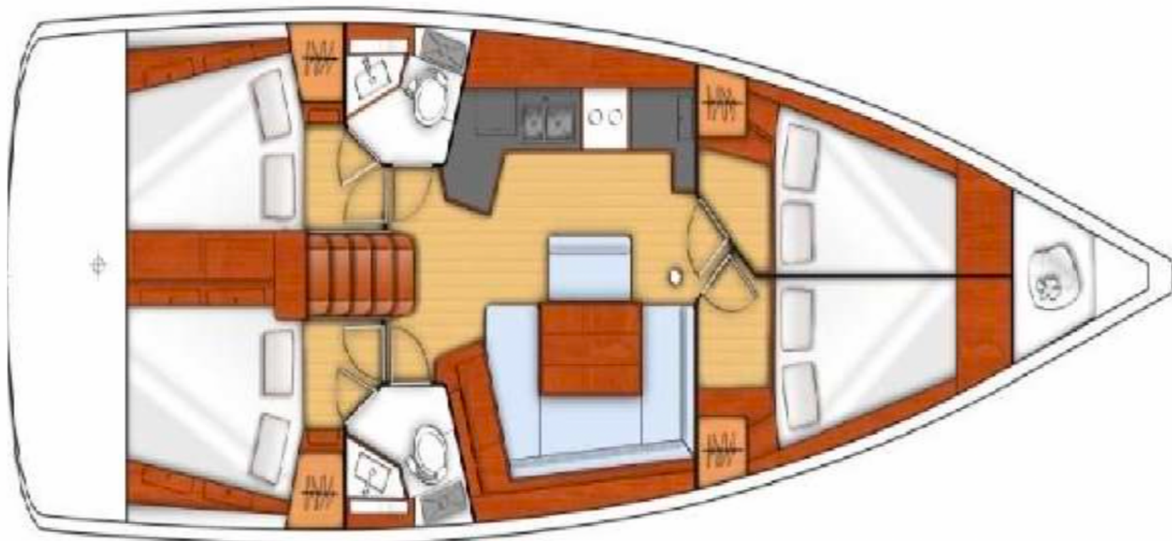
VERSION 4 CABINS / 2 TOILETS
